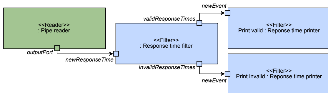
Figure 4.1: Example pipe-and-filter configuration
