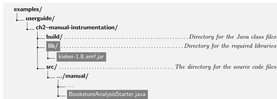
Figure 2.7: Directory layout of the example application with the analysis files highlighted
